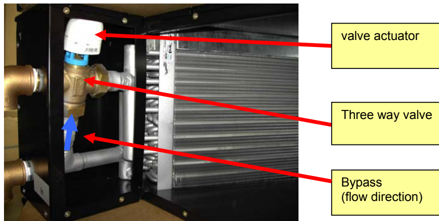
CoolTherm Heat Exchanger (rear view)
